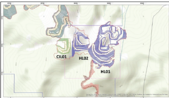
Desain Pit CIL01
